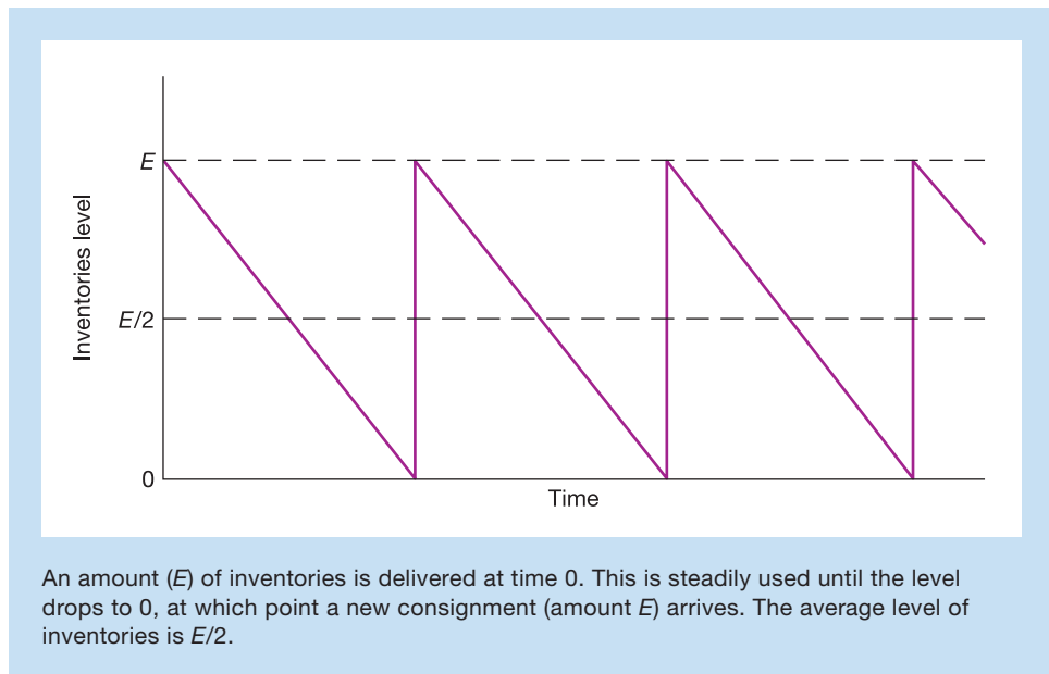
Figure 13.4 Graph of the inventories level against time for an inventory item
